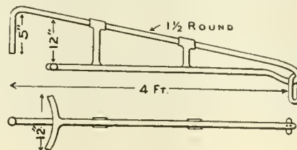
SMOKE STACK CRANE.
